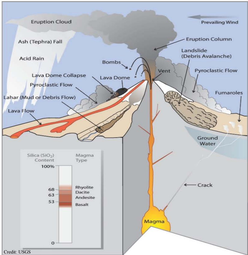
Figure 6-10: Eruption Features
