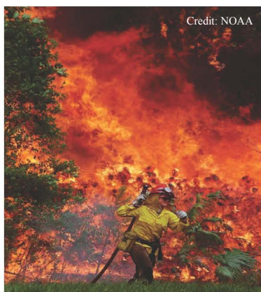
Figure 6-7: Wildfire
